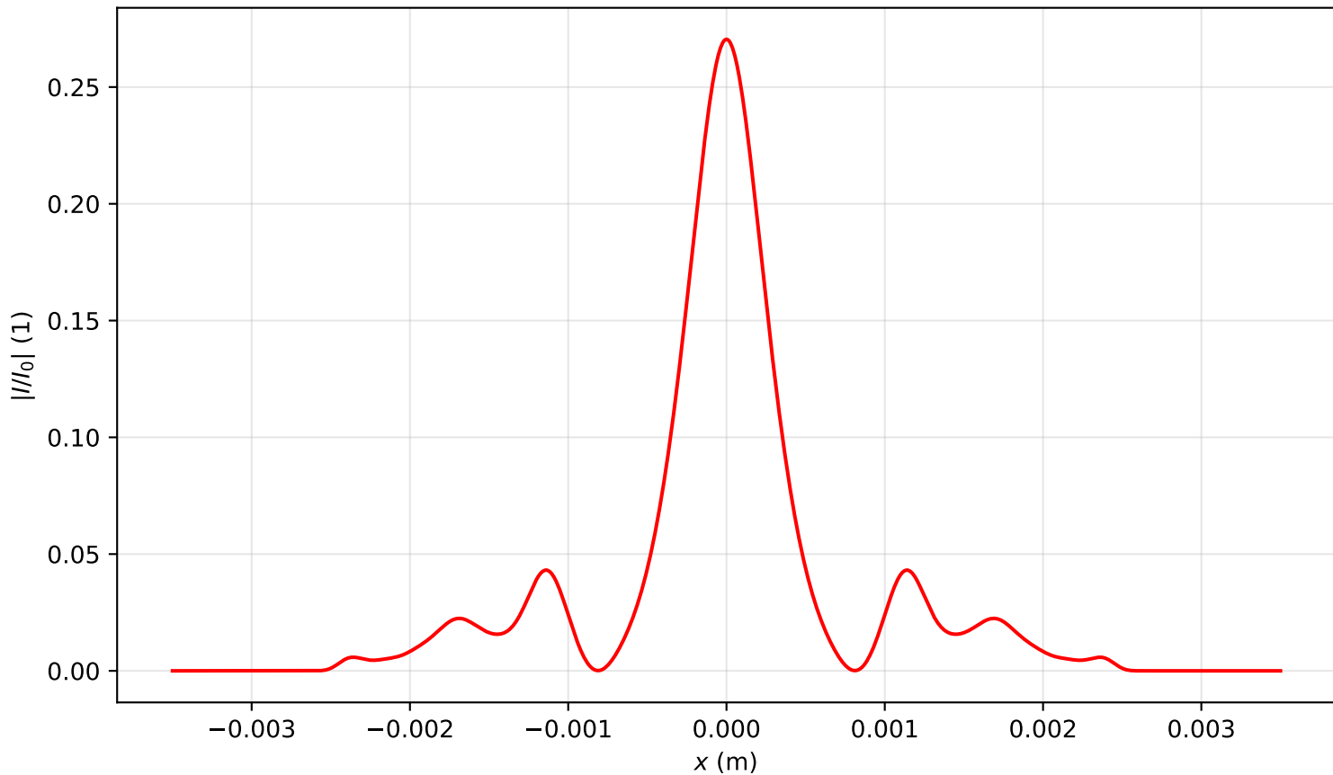
Intensity profile I(x, y = 0, z = 3.821)/I_0 , P_{in}=8.0P_{cr} , artificial time
